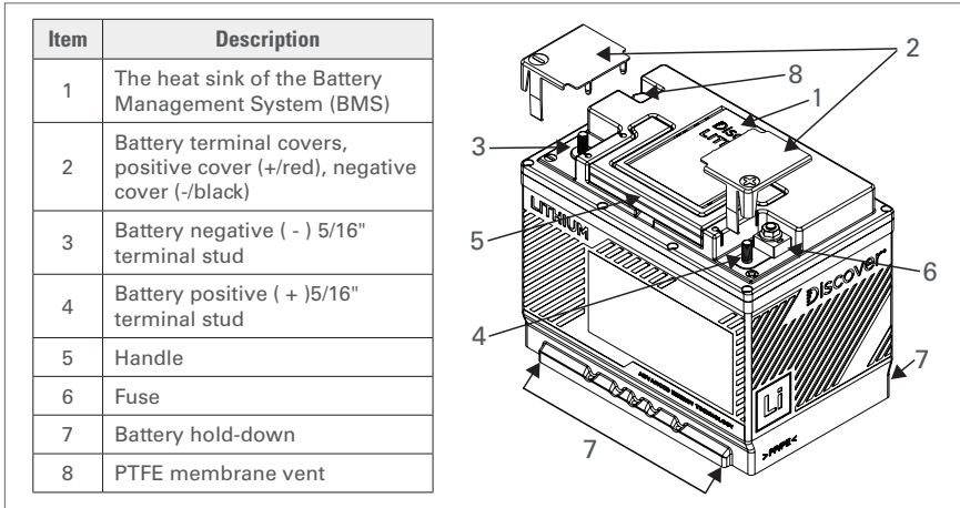
Figure 1. Battery Features.
