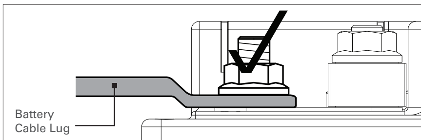
Figure 2. Correct Installation.
