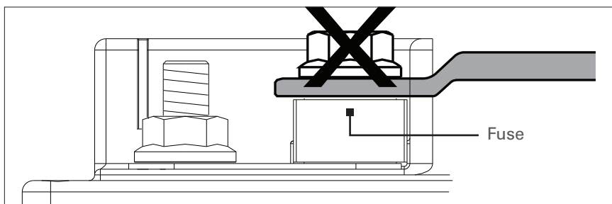
Figure 3. Incorrect Installation.
